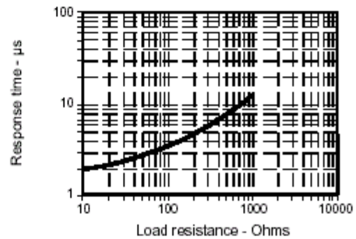
Fig. 4 Non-Saturated Switching Time vs Load Resistance gra_074.d44
