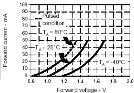
Fig. 3 IRED Forward Bias Characteristics gra_073.d44
