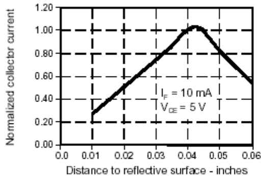
Fig. 1 Normalized Light Current (I L ) vs Distance to Reflective Surface gra_071.d44
