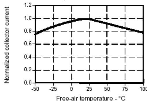
Fig. 6 Collector Current vs Ambient Temperature gra_076.d44
