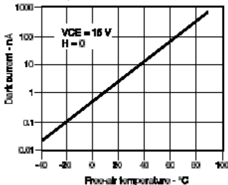
Fig. 5 Dark Current vs Temperature gra_301.d44
